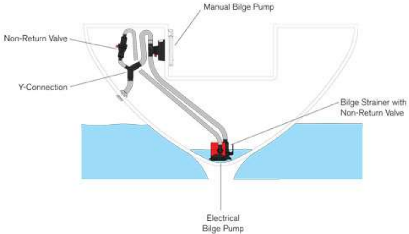
Bilge Pump System
